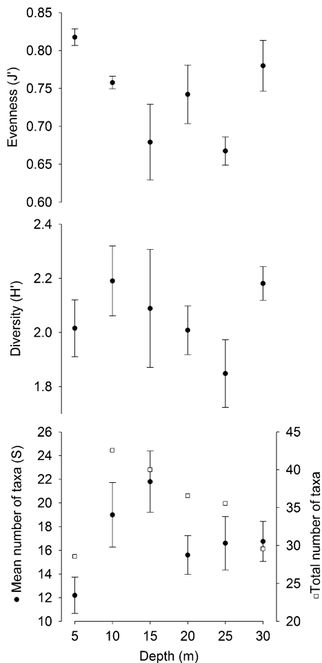
Fig. 3 Evenness ( J' ), Shannon diversity ( H' , \log e ) as well as mean (filled circle) and total (open square) number of taxa of macrobenthos at six different depths (5–30 m) of the soft bottom habitat Brandal (Kongsfjorden, Spitsbergen)
